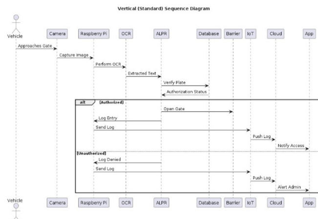
Fig 5. Sequence Diagram
