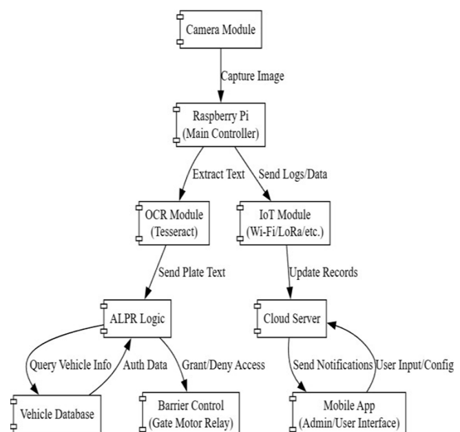
Fig 3. Block Diagram
