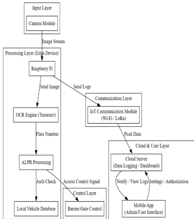
Fig 4. System Architecture
