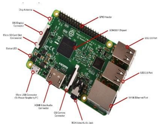
Fig 8. Raspberry Pi Module
