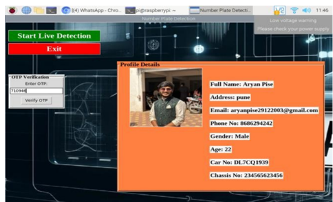
Fig 12. OTP Generation
