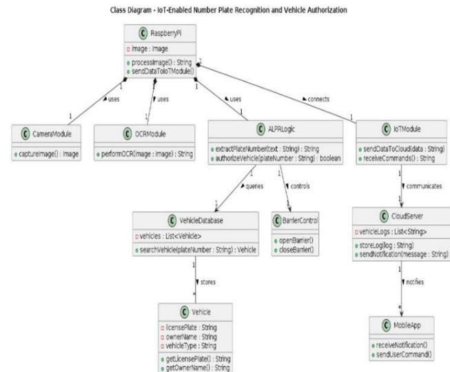
Fig 7. Class Diagram
