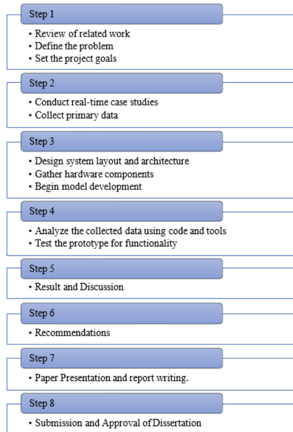
Fig 2. Research Methodology
